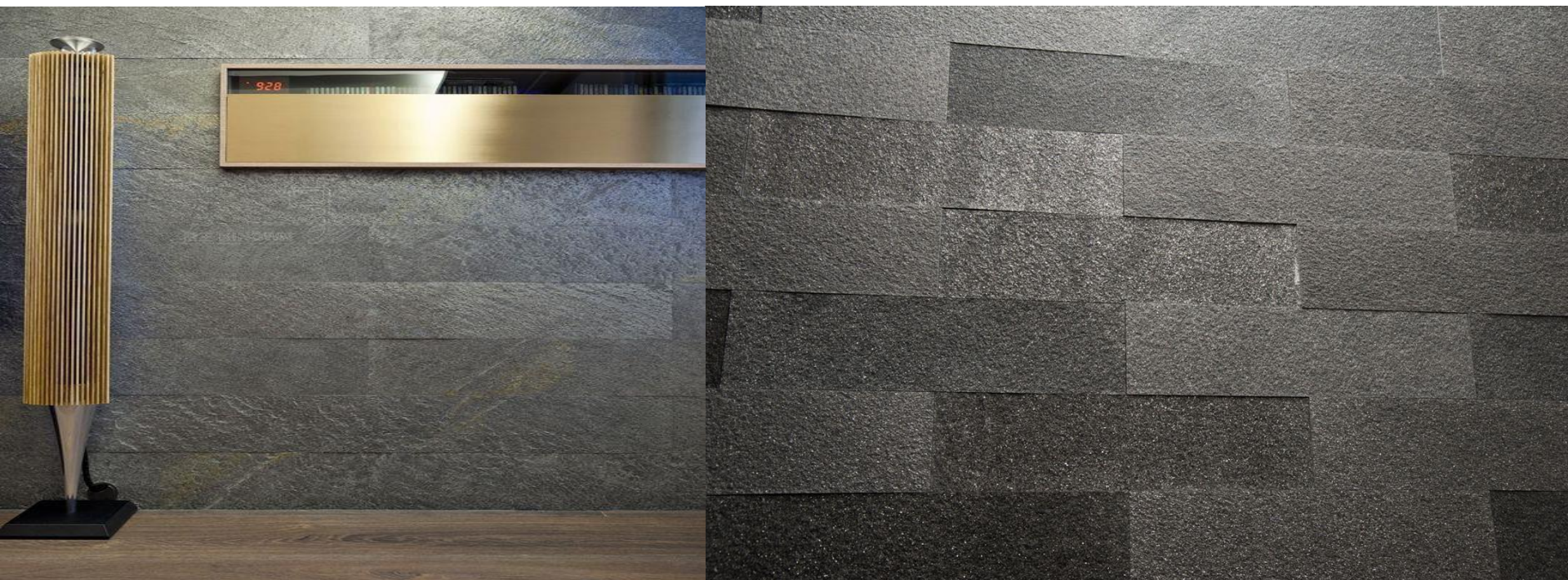
OWL Star Galaxy
